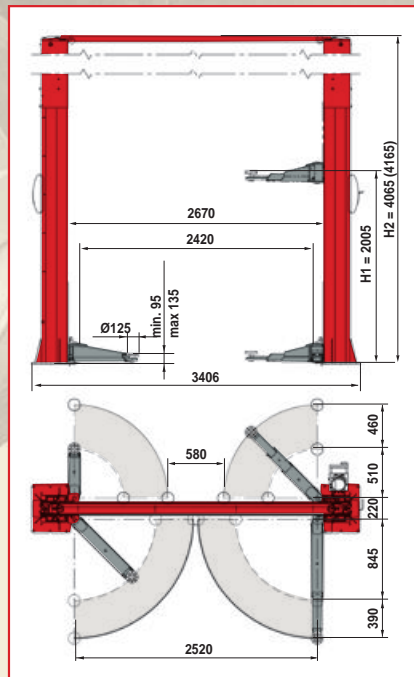
HYDROS 70.42K / 70.45KEX
