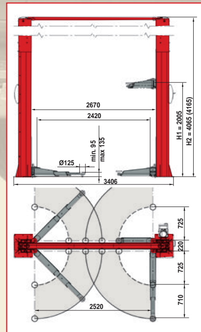
HYDROS 70.42LIK / 70.45LIKEX
